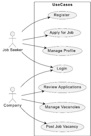
Picture 2. Use case diagram
