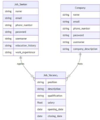
Picture 3. Entity Relationship Diagram
