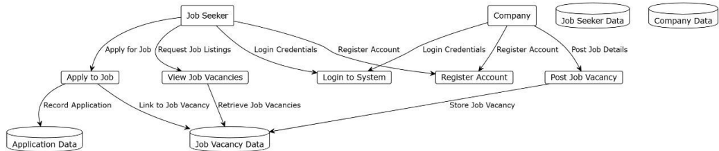
Picture 4. Data Flow Diagram
